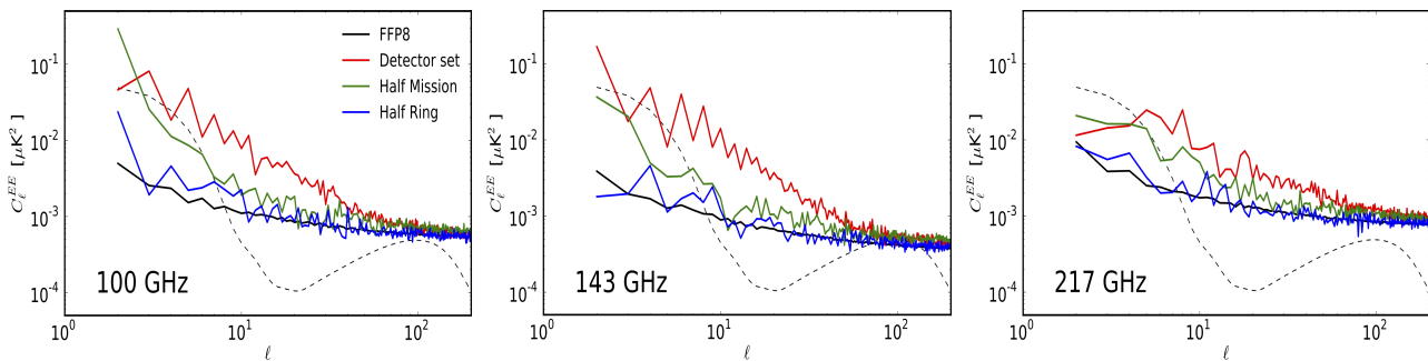
Figure 3.11: EE power spectra reconstructed from the half-difference between data subset maps for the dipole-calibrated channels at low multipoles compared to the noise estimation from the FFP8 simulations. CMB signal from Planck 2015 is plotted in dashed lines.
