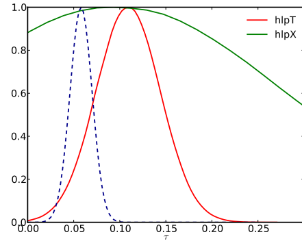
Figure 7.6: Posterior distribution for the reionization optical depth \tau for HillipopT (red line) and HillipopX (green line) compared to the prior from Planck Collaboration Int. XLVII (2016) used throughout this analysis (dashed darkblue line).
