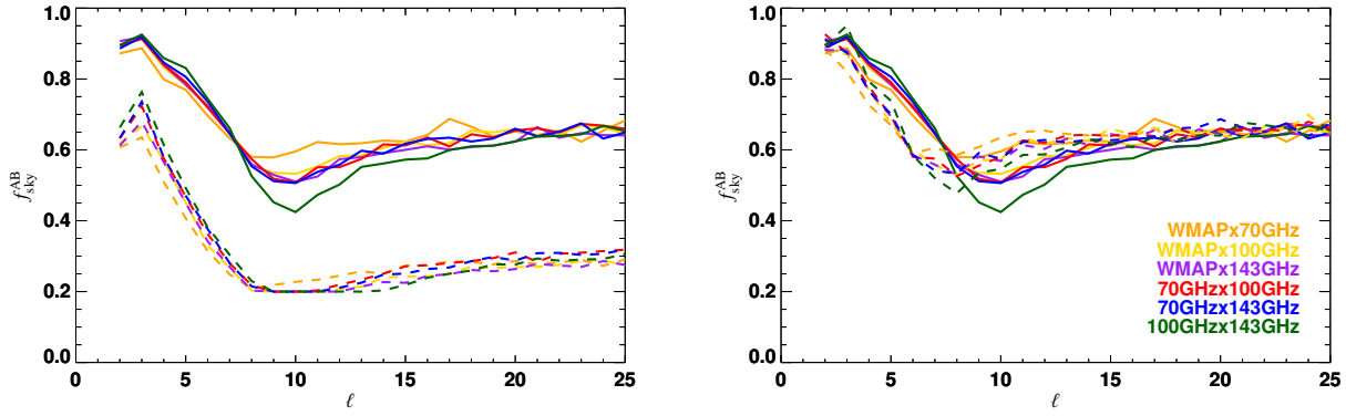
Figure 5.4: Left panel: Dependence of the f_{\text{sky}}^{A \times B} factor on the mask. The two distinct groups (full and dashed lines) represents the f_{\text{sky}}^{A \times B} values fitted to the distributions obtained respectively on the small mask ( f_{\text{sky}} = 0.77 ) and large ( f_{\text{sky}} = 0.49 ) mask. Right panel: Dependence of the f_{\text{sky}}^{A \times B} factor on the fiducial model. The plot shows the f_{\text{sky}}^{A \times B} factor as a function of the multipole when the early-reionization model (model 1, \tau=0.09 , solid lines) and the late-reionization model (model 2, \tau=0.056 , dashed lines) are used as input cosmology in the simulations.
