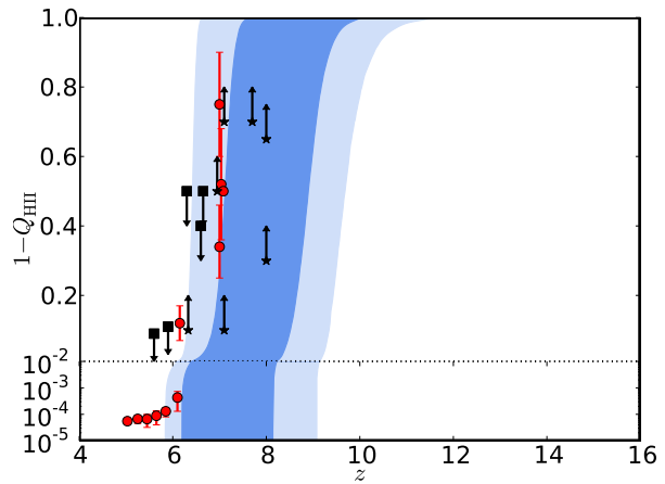
Figure 9.17: Reionization history for the redshift-symmetric parameterization compared with other observational constraints coming from quasars, Ly- \alpha emitters, and the Ly- \alpha forest (compiled by Bouwens et al. 2015). The red points are measurements of ionized fraction, while black arrows mark upper and lower limits. The dark and light blue shaded areas show the 68 % and 95 % allowed intervals, respectively.
