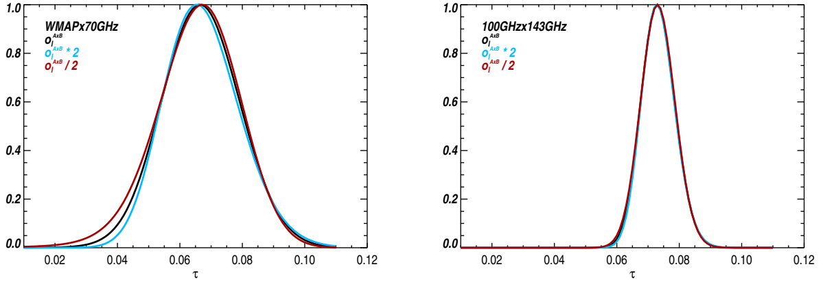
Figure 5.10: The plots show the effect of changing the offsets amplitude by a factor of two on the posterior distribution of the \tau parameter. The left panel refers to the WMAP \times Planck-70 cross-spectra, while the right panel to the Planck-100 \times Planck-143 cross-spectra.
