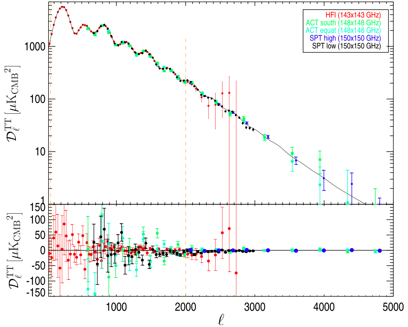
Figure 8.6: Foreground-subtracted CMB cross-spectra of all the experiments used at \approx 150 GHz. The solid line is the best fit of the Hillipop+VHL combination and is subtracted to obtain the bottom residual plot. The Hillipop likelihood uses individual multipoles up to 2000 and window functions have been accounted for in the VHL data.
