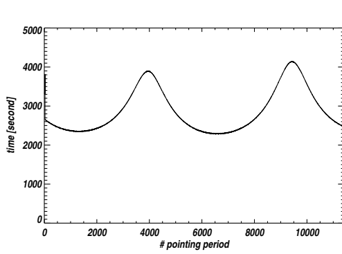
Figure 1.1: Dwelling time of the simulated stable pointing periods for the 12.5 month-long observation. The variation in the period length reflects that the spin axis does not remain in the Ecliptic plane but follows a cycloid path.
